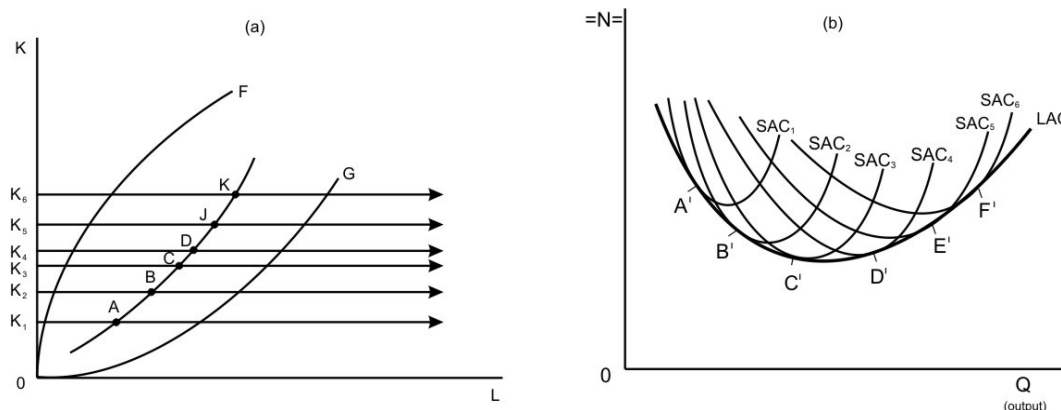
Figure 3.2 Relation between Plant Size, the expansion Path, and the Long-Run Average Cost “Envelope Curve”
