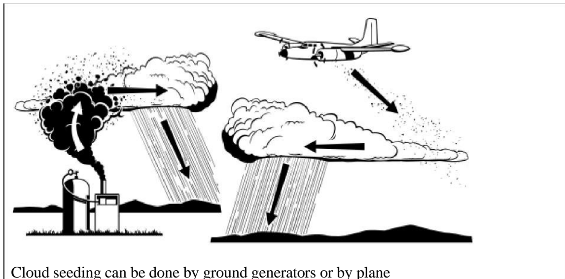
Figure 1.1. Cloud Seeding
