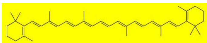
-Carotene
