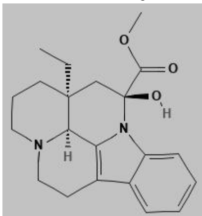
atropine
