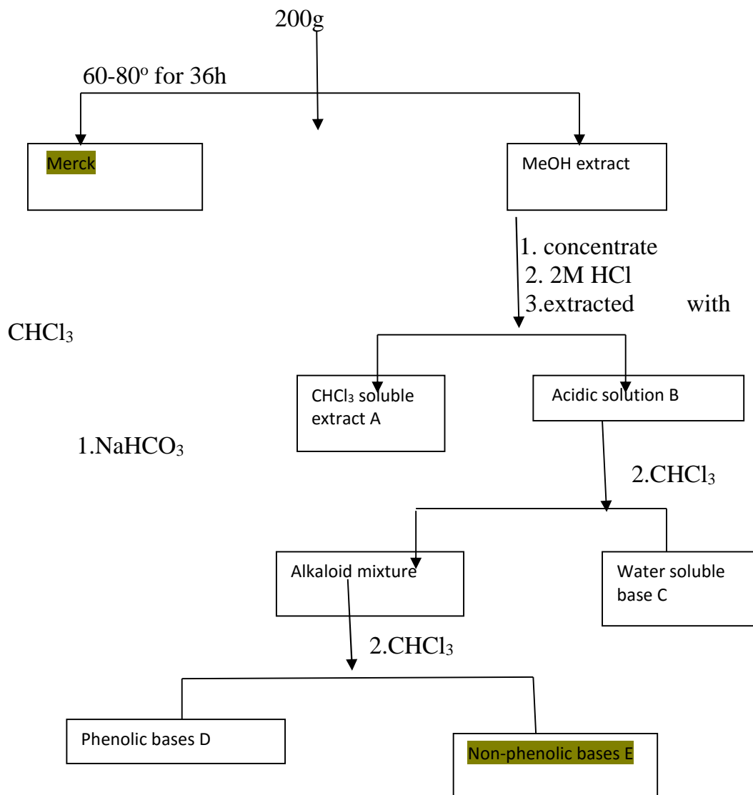
Scheme 1: Extraction and Isolation of Alkaloids from Plant Material Using Methanol as Solvent
