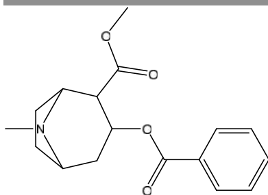
cocaine
