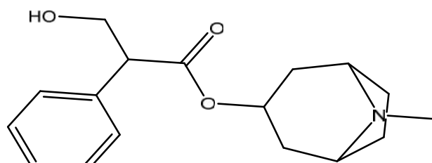
atropine
