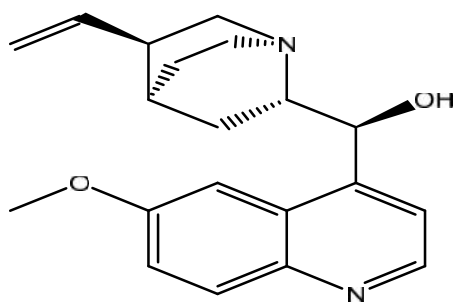
quinidine
