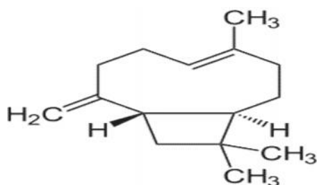
caryophyllene
