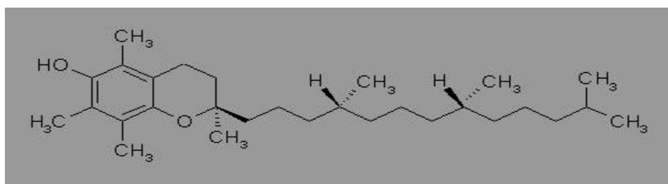
– Tocopherol
