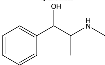
ephedrine
