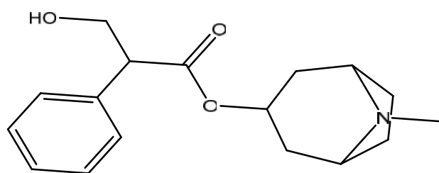
atropine
