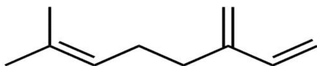
Myrcene
