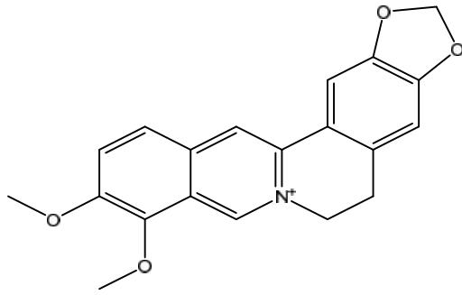
berberine
