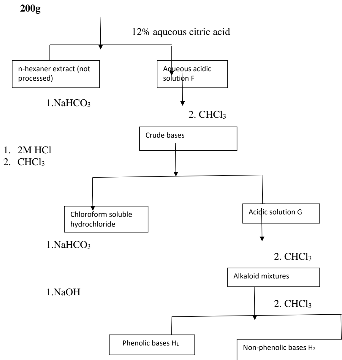
Scheme 2: Extraction and Isolation of Alkaloids from Plant Material Using n- Hexane as Solvent
